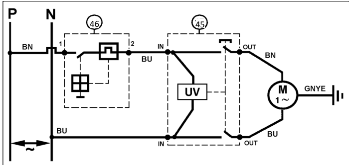
SCHEMA ELECTRIQUE
